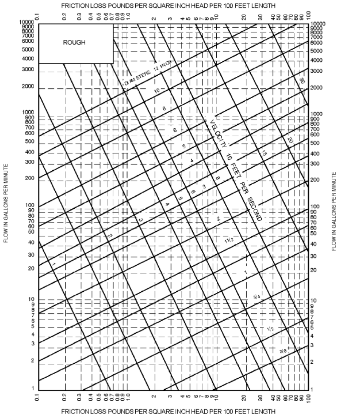
FIGURE E103.3(6) FRICTION LOSS IN ROUGH PIPE a
