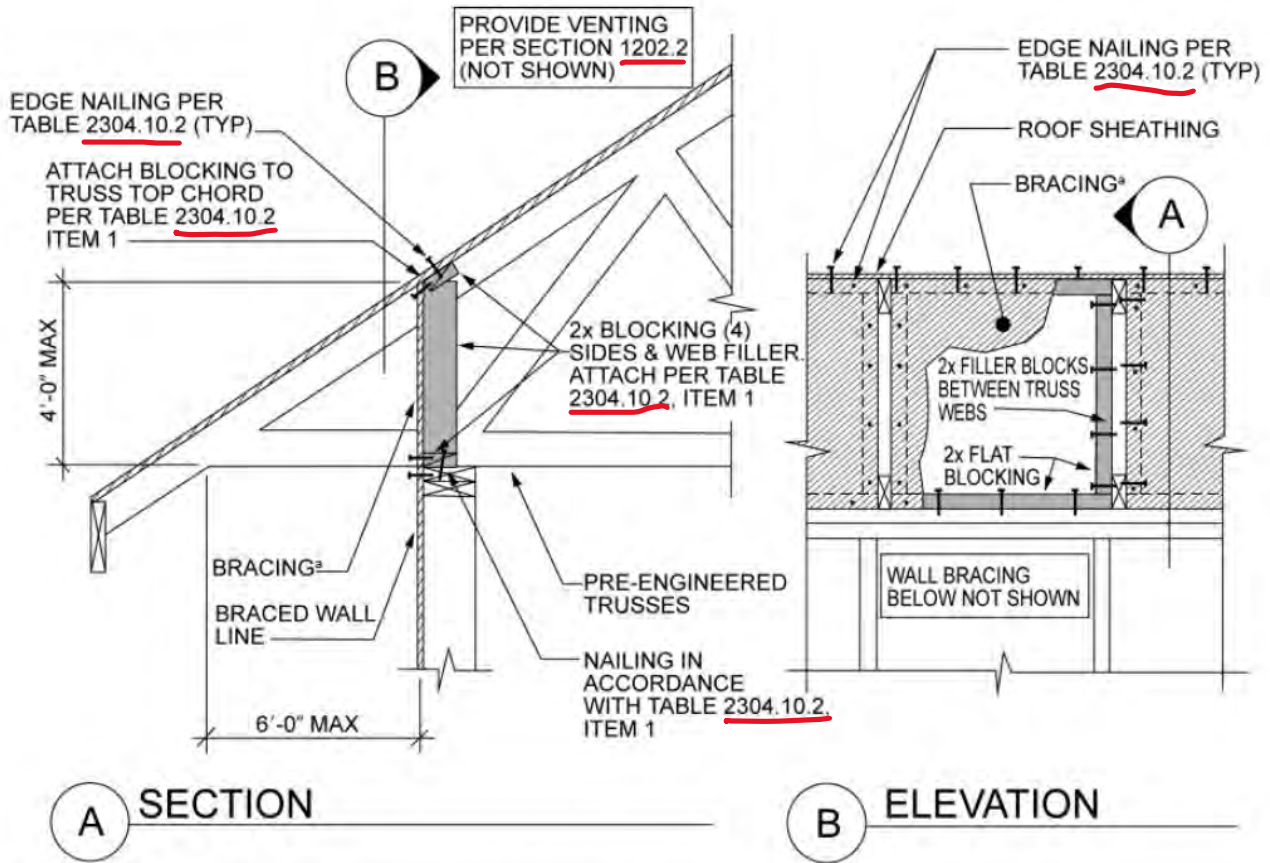
For St: 1 foot = 304.8 mm. a. Methods of bracing shall be as described in Table 2308.6.3(1) DWB, WSP, SFB, GB, PBS, PCP or HPS. FIGURE 2308.6.7.2(2) BRACED WALL PANEL TOP PLATE CONNECTION
