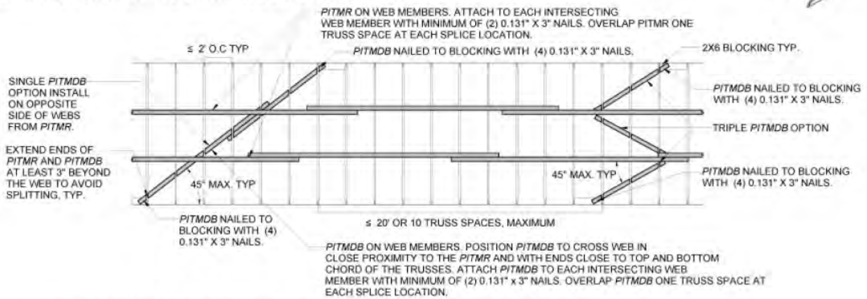
FIGURE 2303.4.1.2(3) PITMR AND PITMDB FOR TRUSS WEB MEMBERS REQUIRING TWO ROWS OF PITMR
