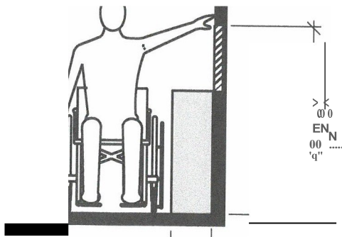
10 max / 255 FIGURE 308.3.2(A) OBSTRUCTED HIGH SIDE REACH
