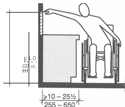
FIGURE 1104.9 REACH OVER A KITCHEN OR BATHROOM CABINET
