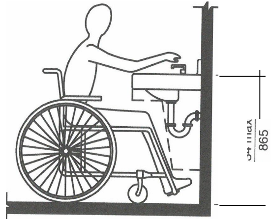
FIGURE 606.3 HEIGHT OF LAVATORIES AND SINKS
