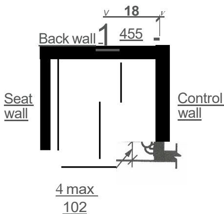
FIGURE 608.3.1(6) GRAB BARS IN TRANSFER-TYPE SHOWER - PLAN
