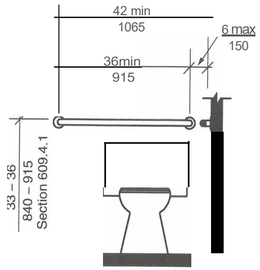
FIGURE 604.5.2
