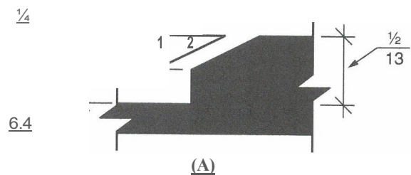
FIGURE 303.2 VERTICAL CHANGE IN LEVEL
