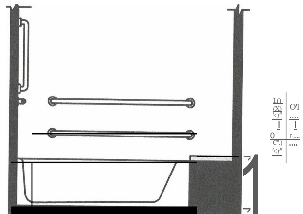
FIGURE 610.2(8) BATHTUB SEATS SEAT PROVIDED AT HEAD END OF TUB
