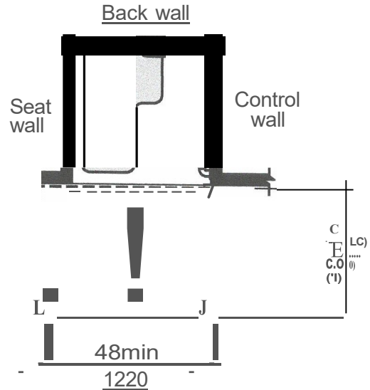
FIGURE 608.2.1.2(C)
