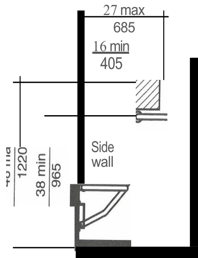
FIGURE 608.4.3(A)
