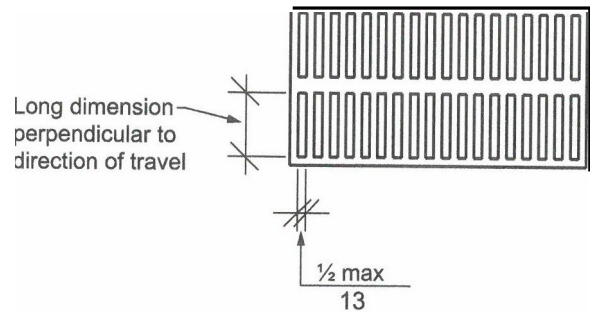
FIGURE 302.3 OPENINGS IN FLOOR SURFACES
