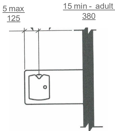
FIGURE 602.2.4 WHEELCHAIR DRINKING FOUNTAIN SPOUT LOCATION
