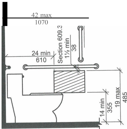
FIGURE 604.11.7(A) CHILDREN'S DISPENSER OUTLET LOCATION
