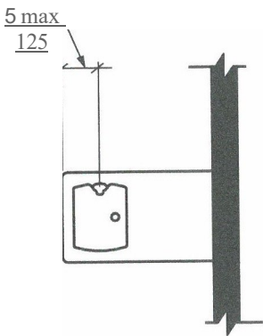
FIGURE 602.3.3 STANDING USE DRINKING FOUNTAIN SPOUT LOCATION
