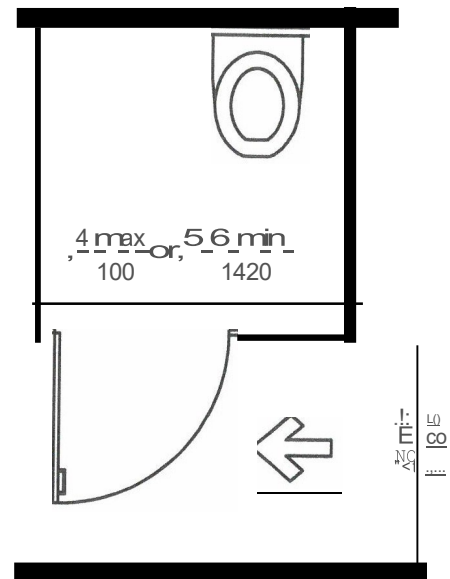
FIGURE 604.9.3.1(A) WHEELCHAIR TOILET COMPARTMENT DOOR OPENING LOCATION • DOOR SWINGING IN ON FRONT WALL OF PARTITION
