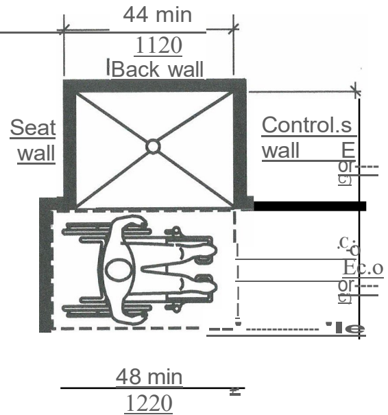
FIGURE 1104.11.3.1.3.3(6) TRANSFER-TYPE SHOWER COMPARTMENT IN TYPE B UNITS EXCEPTION
