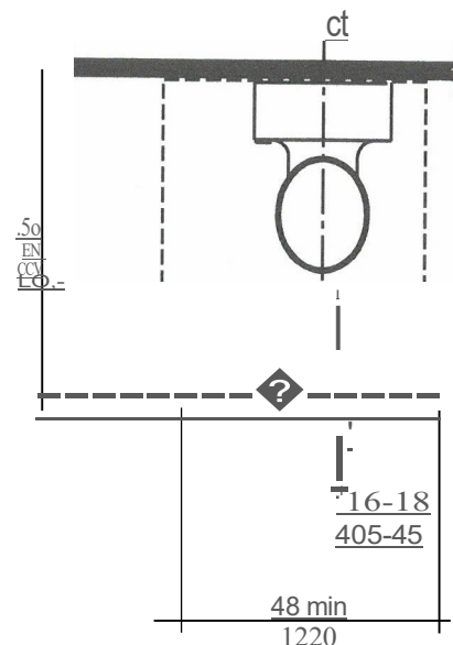
FIGURE 1104.11.3.1.2(8) CLEARANCE AT WATER CLOSETS IN TYPE B UNITS CLEARANCE WIDTH AND DEPTH
