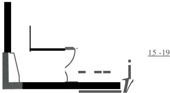
FIGURE 1103.11.2.4(0) WATER CLOSETS IN TYPE A UNITS: WATER CLOSET SEAT HEIGHT
