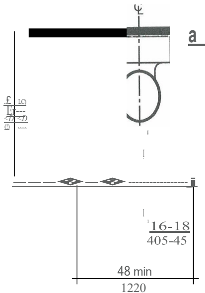
FIGURE 1104.11.3.1.2(C) CLEARANCE AT WATER CLOSETS IN TYPE 8 UNITS INCREASED CLEARANCE DEPTH - FORWARD APPROACH
