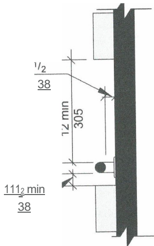
FIGURE 609.3 SPACING OF GRAB BARS
