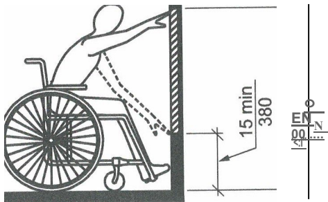
FIGURE 308.2.1 UNOBSTRUCTED FORWARD REACH
