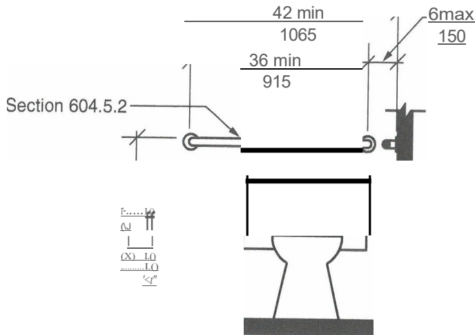
FIGURE 609.4.2(8) POSITIONS OF CHILDREN'S GRAB BARS REAR-WALL VIEW
