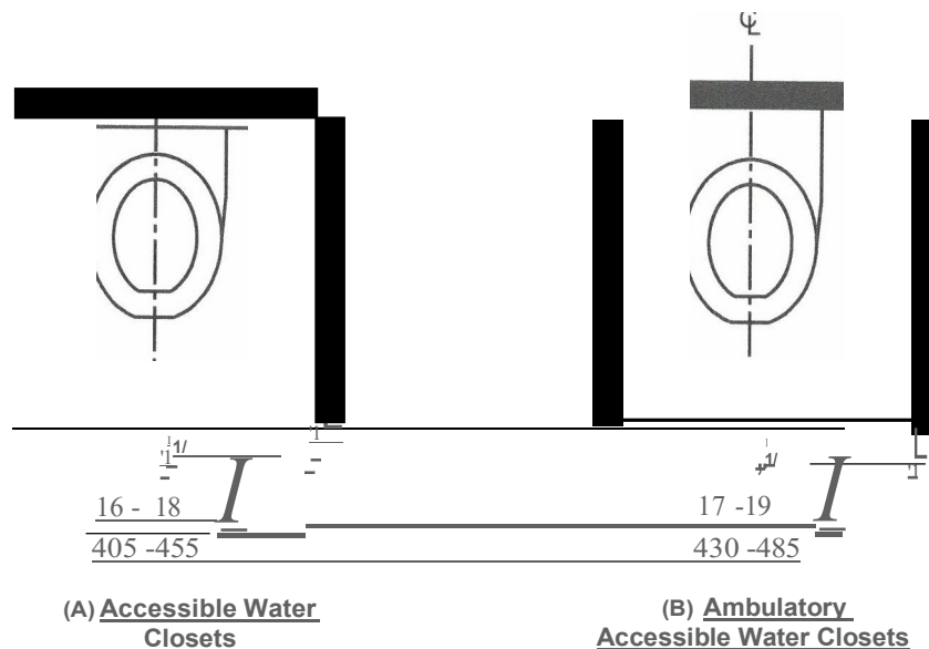
FIGURE 604.2 WATER CLOSET LOCATION
