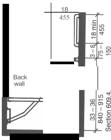
FIGURE 608.3.1(A) GRAB BARS IN TRANSFER-TYPE SHOWER - ELEVATION
