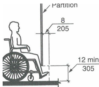
FIGURE 604.9.5(A) TOE CLEARANCE - ELEVATION
