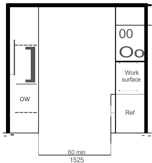
FIGURE 804.2.2(8) U-SHAPED KITCHEN CLEARANCE
