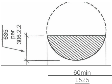
Overlap of knee and toe clearance
