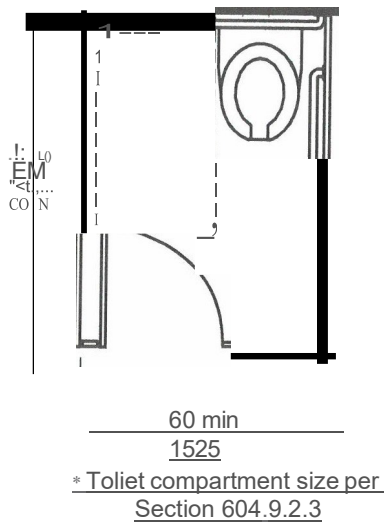
FIGURE 604.9.3(8) WHEELCHAIR TOILET COMPARTMENT DOORS EXCEPTION 3 • ALTERNATE WHEELCHAIR COMPARTMENT
