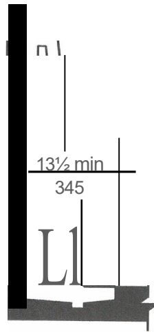
FIGURE 605.2(6) HEIGHT AND DEPTH OF URINAL STALL TYPE
