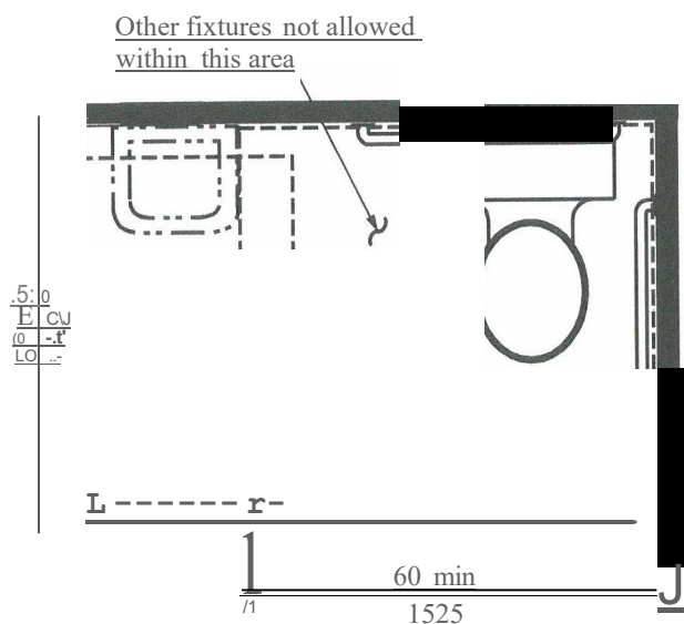
FIGURE 604.3 SIZE OF CLEARANCE FOR WATER CLOSET
