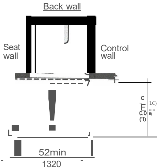
FIGURE 608.2.1.2(A)
