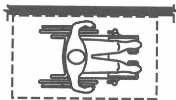
FIGURE 305.5(B) POSITION OF CLEAR FLOOR SPACE - PARALLEL
