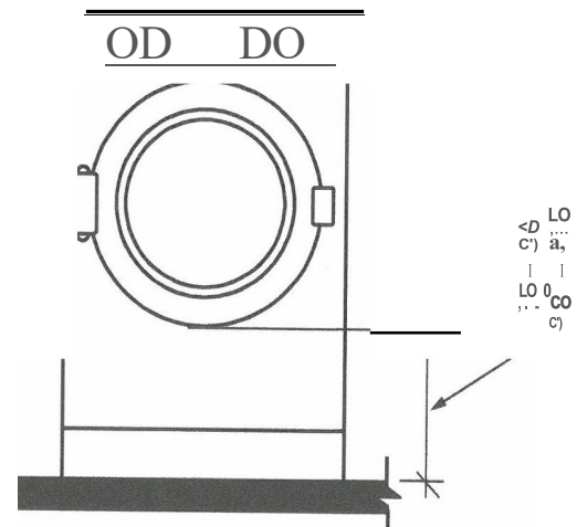
FIGURE 611.4(8) HEIGHT OF LAUNDRY EQUIPMENT • FRONT LOADING
