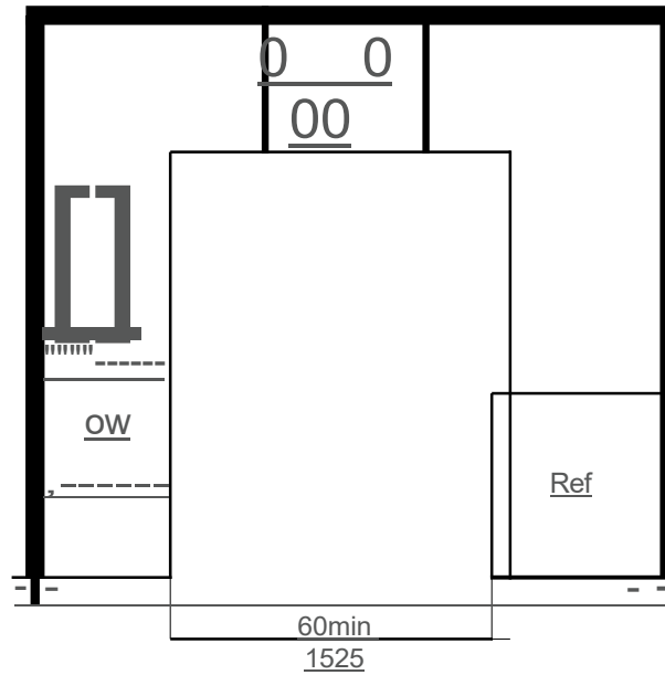
FIGURE 1104.12.1.2(A) LI-SHAPED KITCHEN CLEARANCE IN TYPE B UNITS
