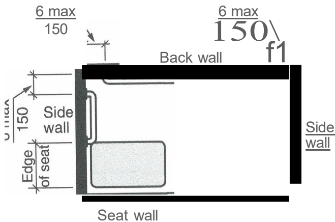
FIGURE 608.3.3(8) GRAB BARS IN ALTERNATE ROLL-IN-TYPE SHOWER - PLAN
