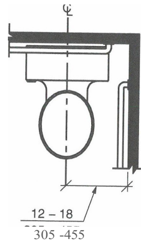
FIGURE 604.11.2 CHILDREN'S WATER CLOSET LOCATION
