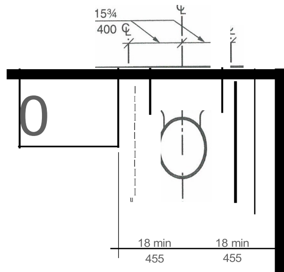
FIGURE 1104.11.1.1 SWING-UP GRAB BARS FOR WATER CLOSETS
