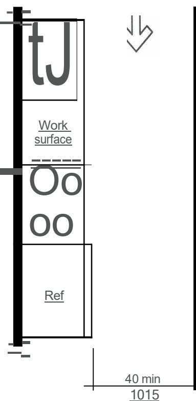
FIGURE 804.2.1(8) PASS-THROUGH KITCHEN CLEARANCE
