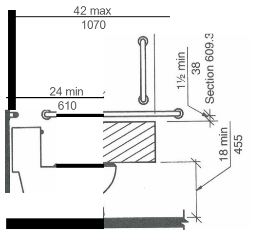
FIGURE 604.7.1(A) DISPENSER OUTLET LOCATION - PROTRUDING DISPENSER BELOW GRAB BAR
