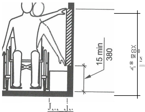
10 max / 255 FIGURE 308.3.1 UNOBSTRUCTED SIDE REACH
