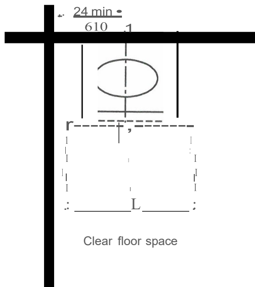
FIGURE 1104.11.3.1.1 LAVATORY IN TYPE B UNITS: OPTION A BATHROOMS
