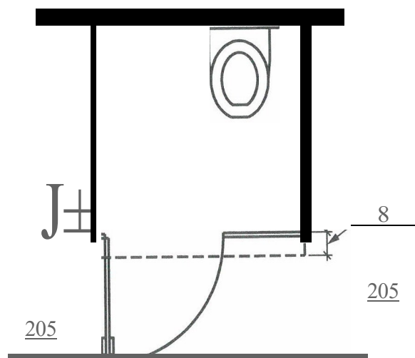
FIGURE 604.9.5(6) TOE CLEARANCE - PLAN
