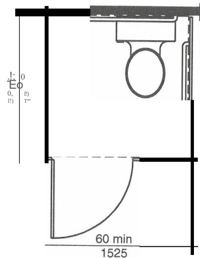
FIGURE 604.9.2(8) WHEELCHAIR TOILET COMPARTMENTS FLOOR MOUNTED WATER CLOSET, ADULT · WALL HUNG AND FLOOR MOUNTED WATER CLOSET, CHILDREN
